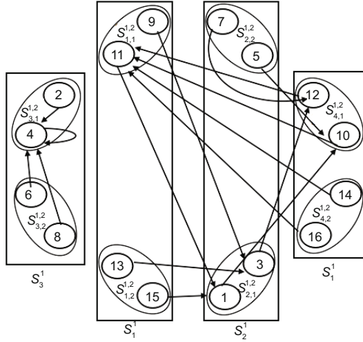
Fig. 4 State transition diagram of \mathcal{G}_3
