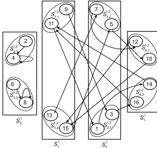
Fig. 5 State transition diagram of \mathcal{G}_4
