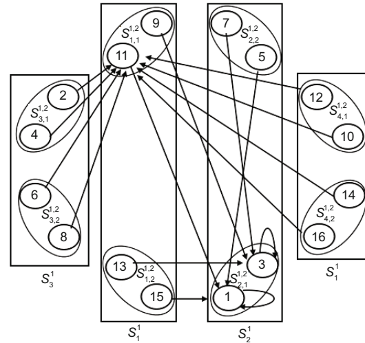
Fig. 2 State transition diagram of \mathcal{G}_1
